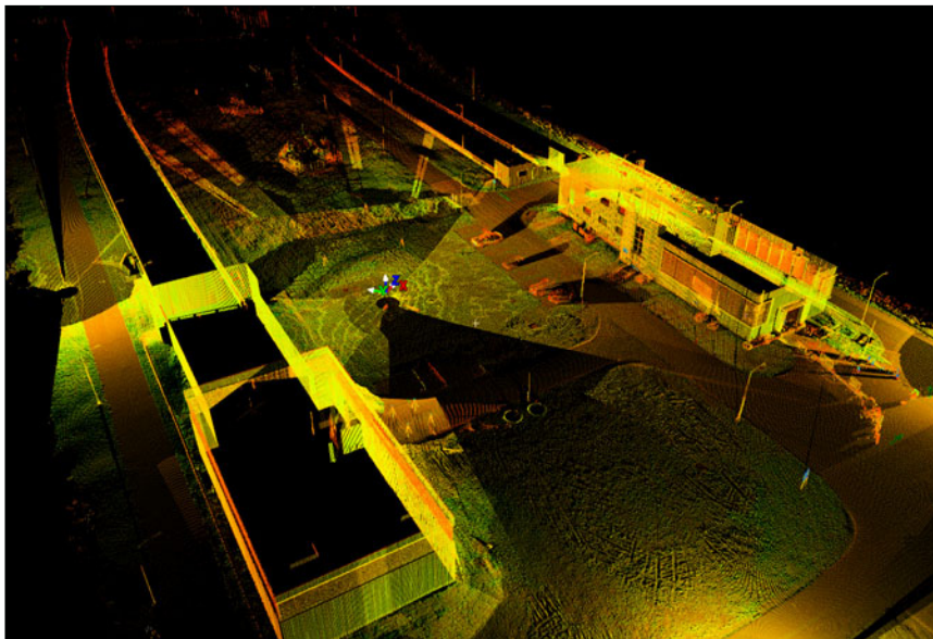
This point cloud image of two of the four ventilation buildings includes the parking area and topographic features.
